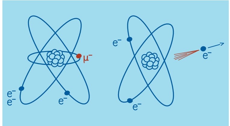
The Mu2e collaboration will capture muons produced by Fermilab’s particle accelerators. If the Mu2e detector records electrons escaping with the precise energy of 105 MeV, scientists will have discovered the elusive transformation of a muon converting directly into an electron — and signs of new physics.
