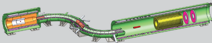
In the Mu2e experiment, muons will be produced in the left section. They will then move through the S-shaped path to the final destination, on the right, where the detector sits. There scientists will look for the telltale sign of a muon converting directly into an electron.
